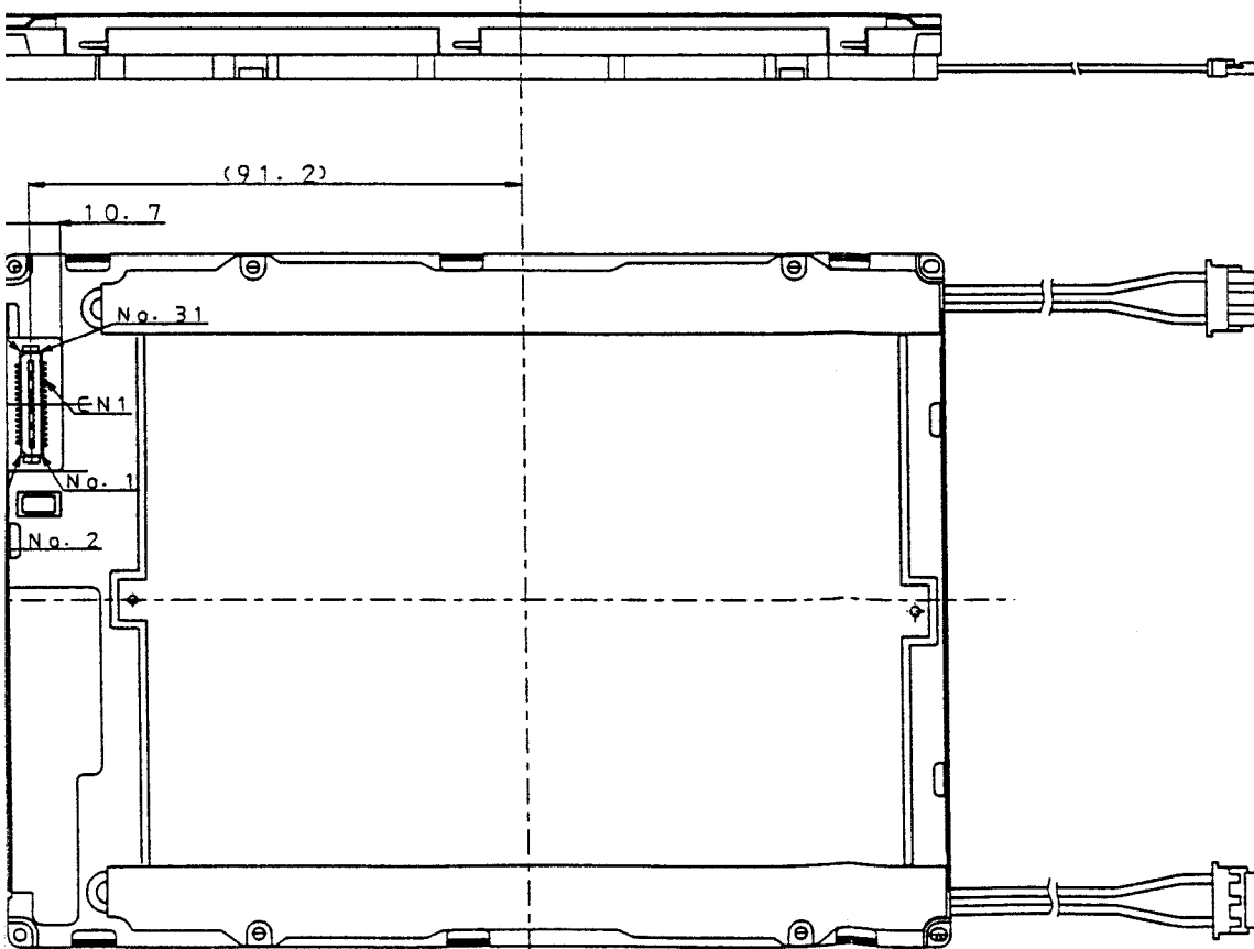
FIG1. LQ64D341 OUTLINE DEMENSIONS
