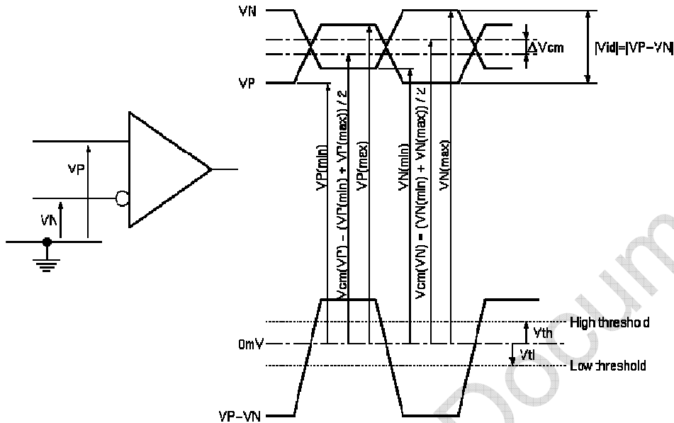
Figure 7 Voltage Definitions
