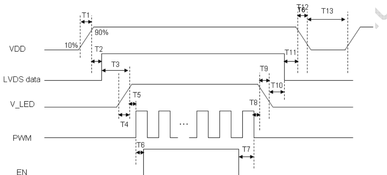
Figure 12 Power Sequence
