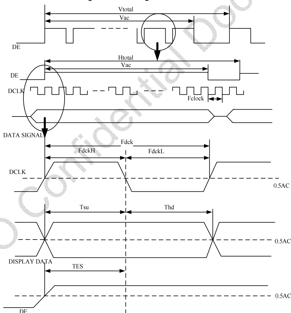
Figure 11 Timing Characteristics
